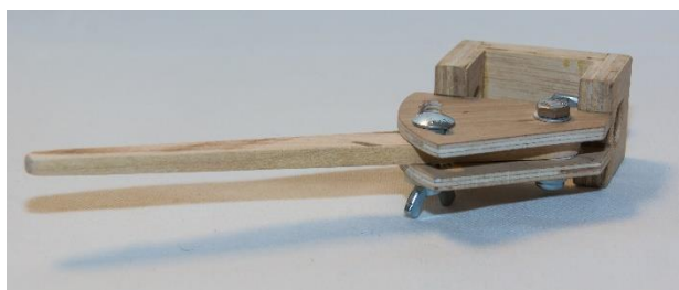
Gouge Grinding Tool by Mikeal Jones
